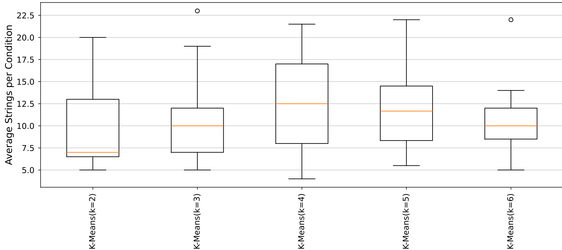
YARA Rules Average Strings per Condition Distribution (Cluster25_Size6 dataset)
